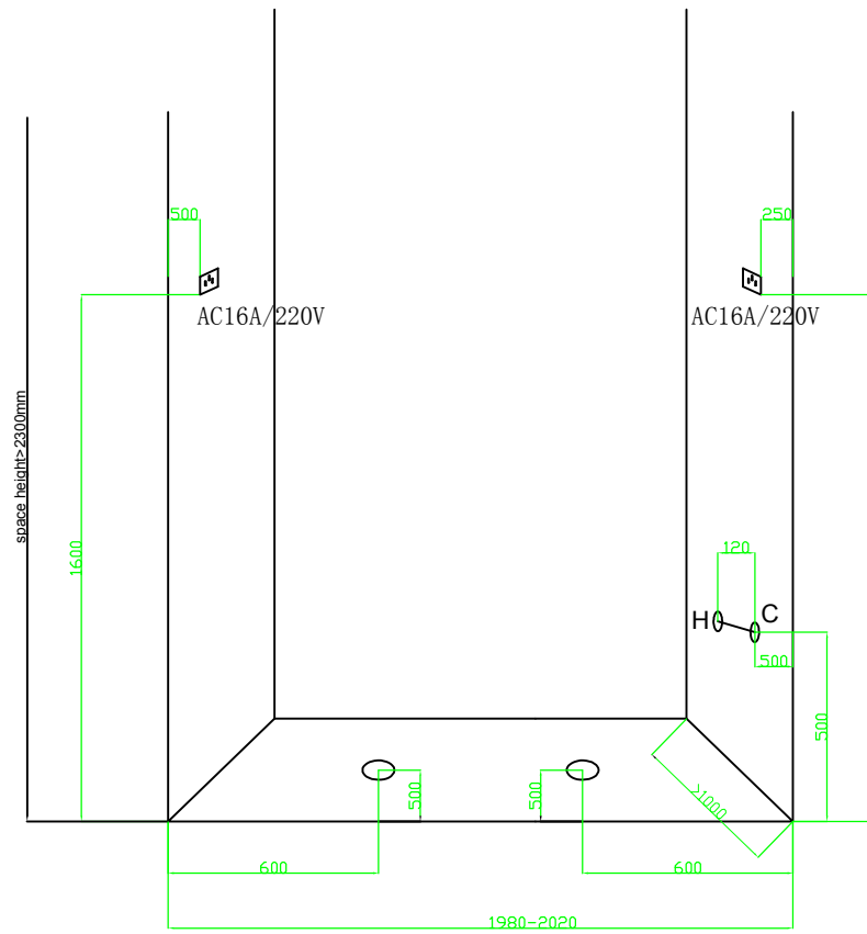
power&water supply for FC2009
