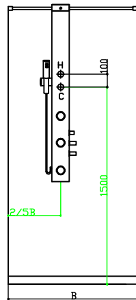
drawing for WR-D2 water and power supply location
