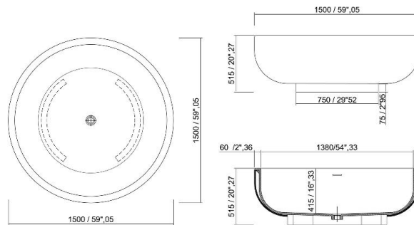
GOLD TUB GLD0102 diametro 1500x515h mm - diameter 59"05x20"27 inches in white Stoneage®
